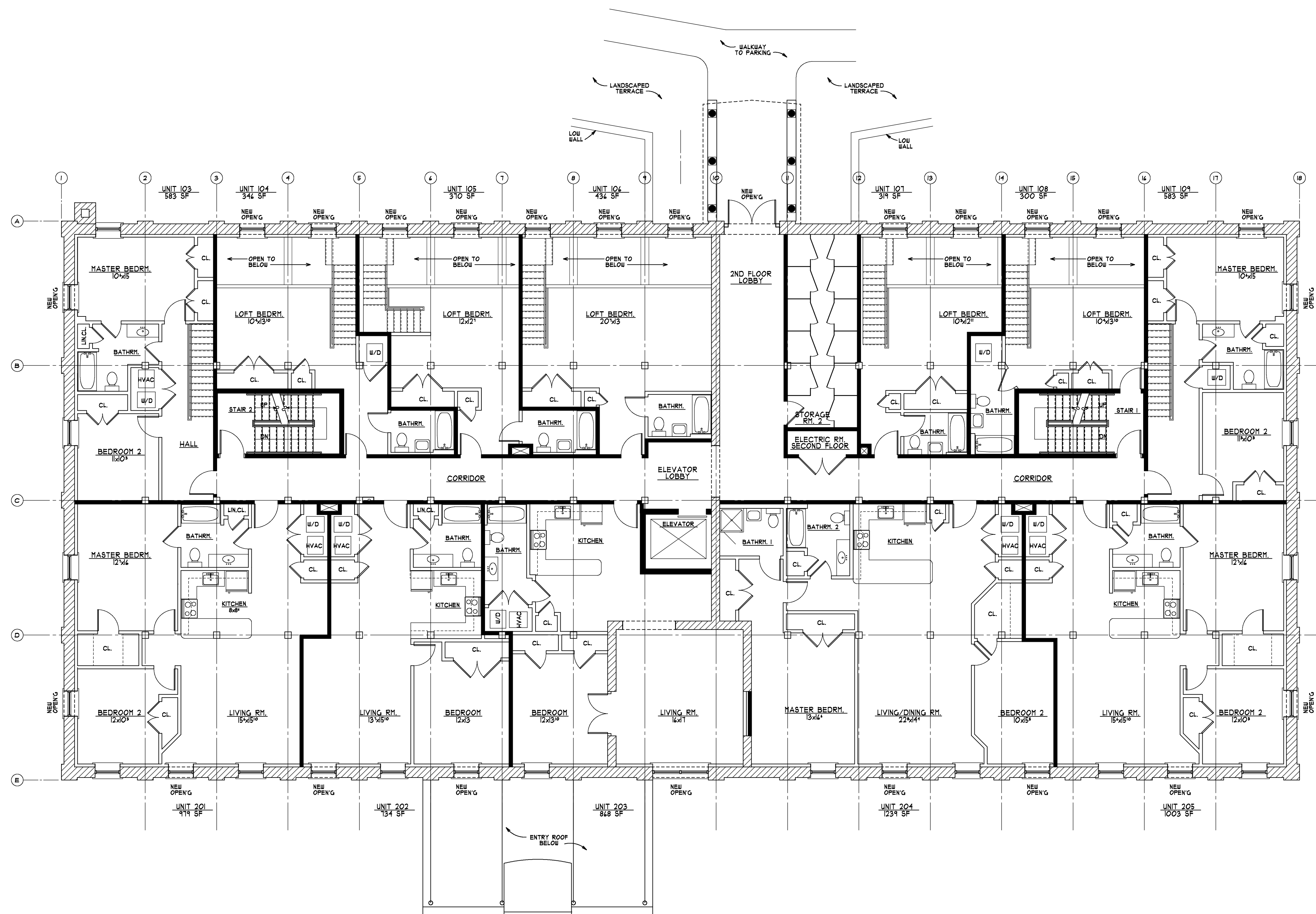
SECOND FLOOR PLAN 1/8" = 1'-0"
