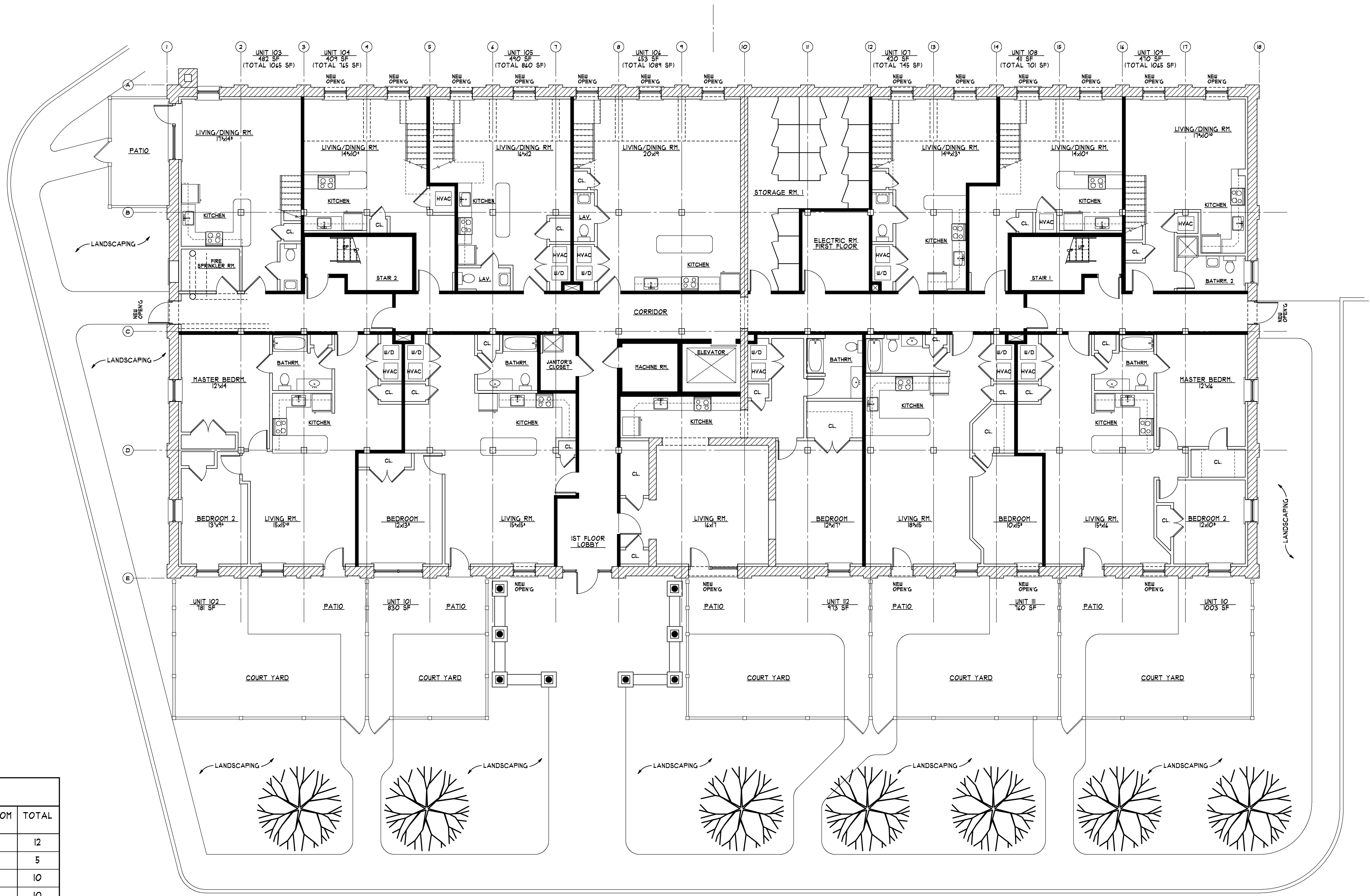
FIRST FLOOR PLAN 1/8" = 1'-0"
